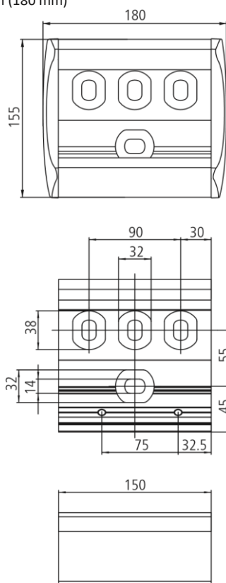
Wall bracket 150 mm (180 mm)
