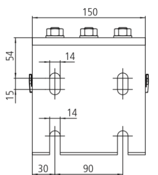
Ceiling angle with wall bracket 150 mm
