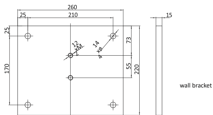
Mounting plate, 260 x 220 x 15 mm + standard
