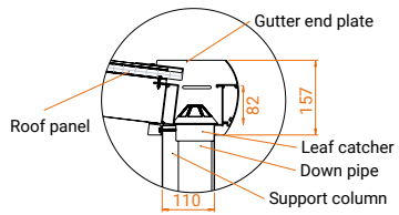
DETAIL A - RADIUS FASCIA
