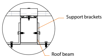
DETAIL D
