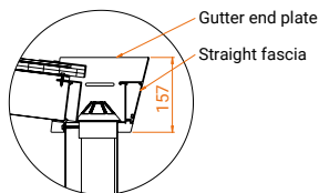
DETAIL A - STRAIGHT FASCIA
