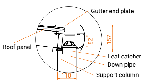
DETAIL A - RADIUS FASCIA
