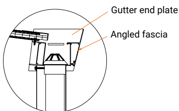
DETAIL A - STRAIGHT FASCIA
